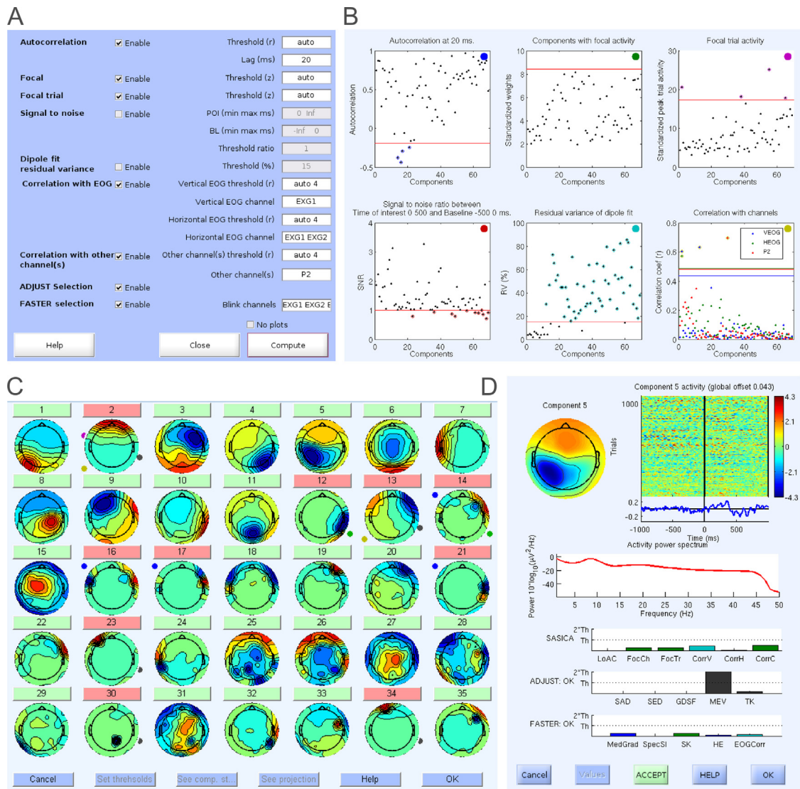
Fig. 1. Graphical user interface. (A) The main graphical interface window allows choosing which methods to use to select components. When pressing the “Compute” button, the plugin computes all enabled methods on the currently loaded EEG dataset and displays the results in separate windows. (B) The first window shows the value of the computed measures (y axis) for all components (x axis). The threshold for selection is shown as a horizontal red line in each panel, and every component that passes the threshold (above or below, according to the measure considered, see text for details) is highlighted in a color specific to the measure being considered, reproduced in the top-right corner of the panel, and used in the window shown in D. A mouse click on any point opens a detailed component properties window. Note that Signal to noise ratio and residual variance are shown in this window here for illustration but were not used to select components in the window shown in (D). (C) In this window, all component topographies are shown, along with a colored button indicating whether a given component is selected for rejection (red) or not (green). Next to the selected components’ topographies, colored dots indicate which computed measure passed threshold. (D) All component properties and measures can be summarized in individual windows, along with the classical EEGLAB plots (topography, single trial time course and power spectrum). All measures are scaled so that larger bars mean that a measure is more likely to select the component for rejection (see Section 2.2.2 for details).
