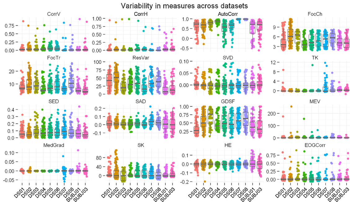
Fig. 7. Measure ranges vary with recording and preprocessing settings.
